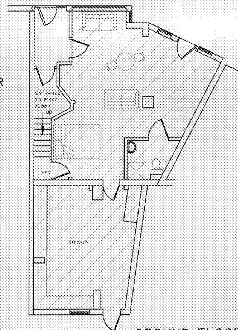
GROUND FLOOR
