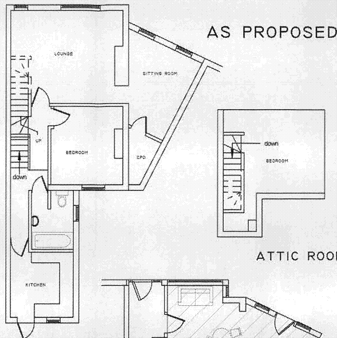
FIRST FLOOR
