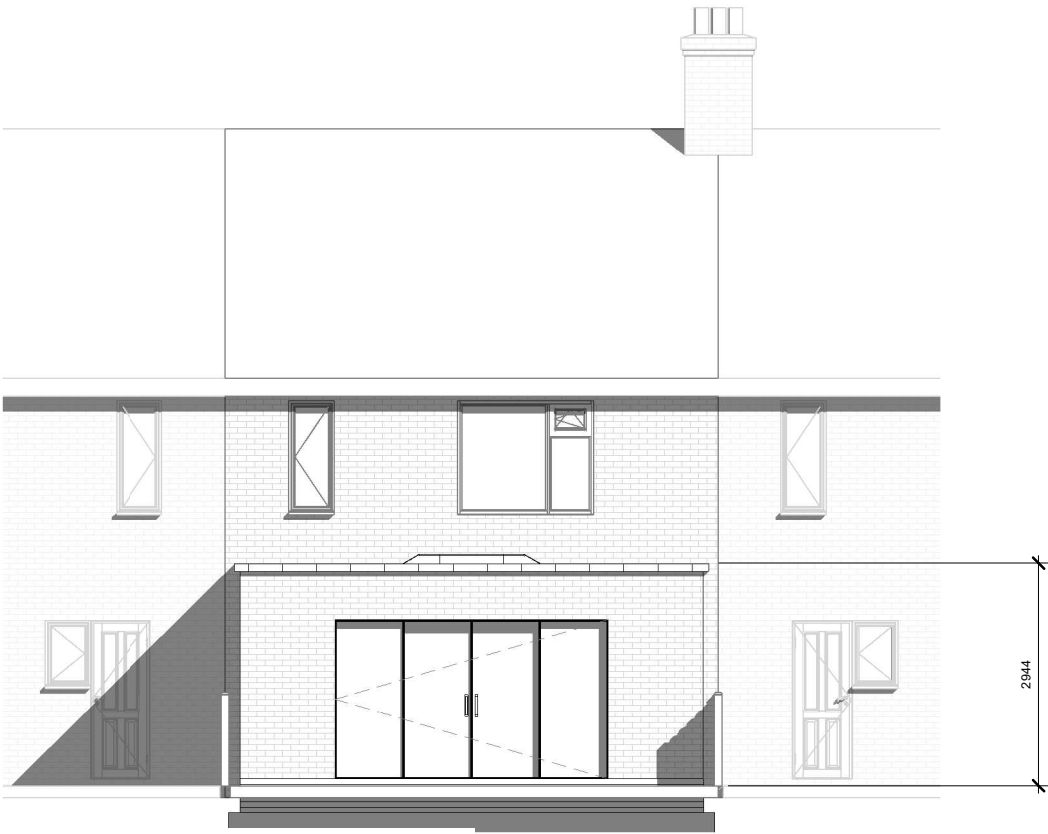
Proposed Elevation-Rear
