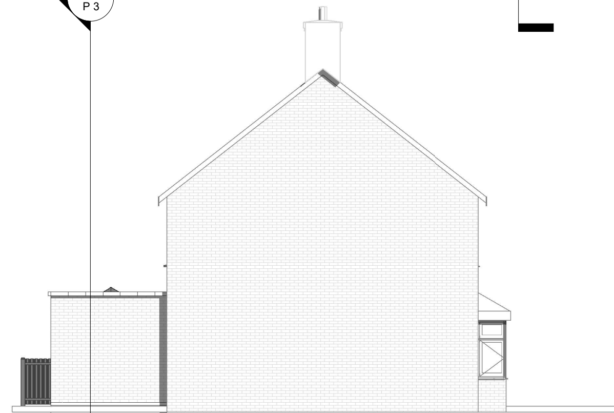
Proposed Elevation-Left side
