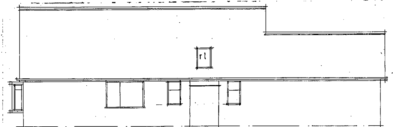
EAST 1/100
