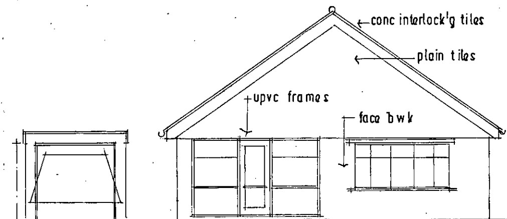
SOUTH [front] 1/100
