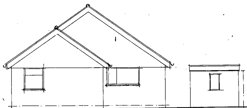
NORTH 1/100
