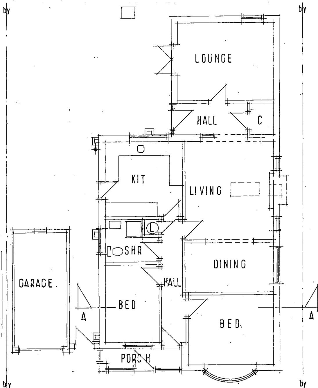
FLOOR PLAN 1/100
