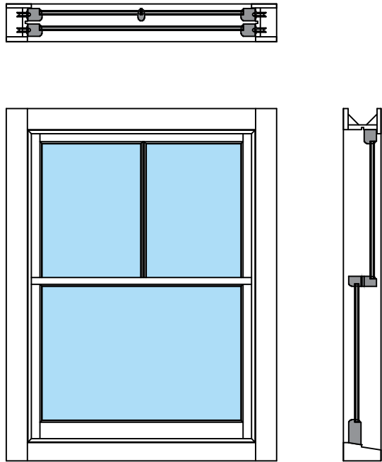
W5 - Kitchen Rear (internal view) Scale 1/20 @ A3
