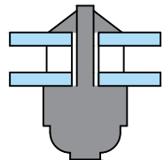
Glazing Bar section
