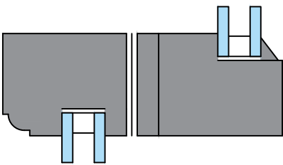
Meeting Rail thru section
