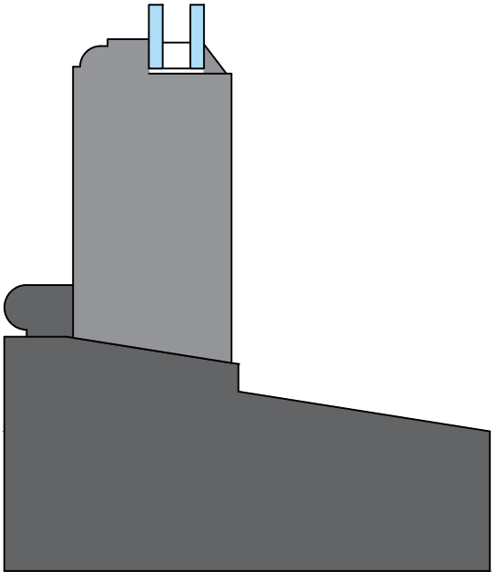
Sill thru section
