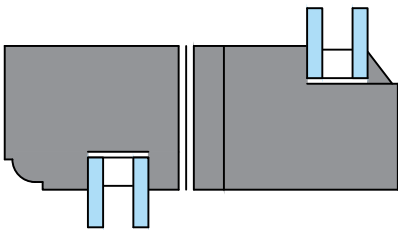
Meeting Rail thru section
