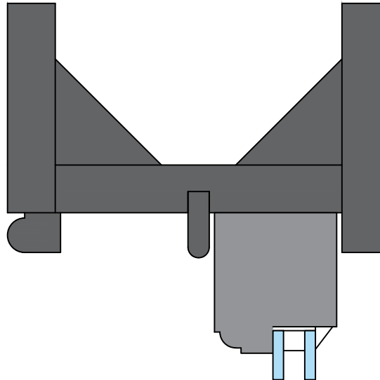
Head thru section
