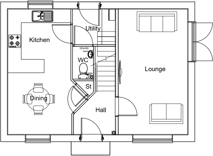
Ground Floor Plan *Obs - Obscured Glass
