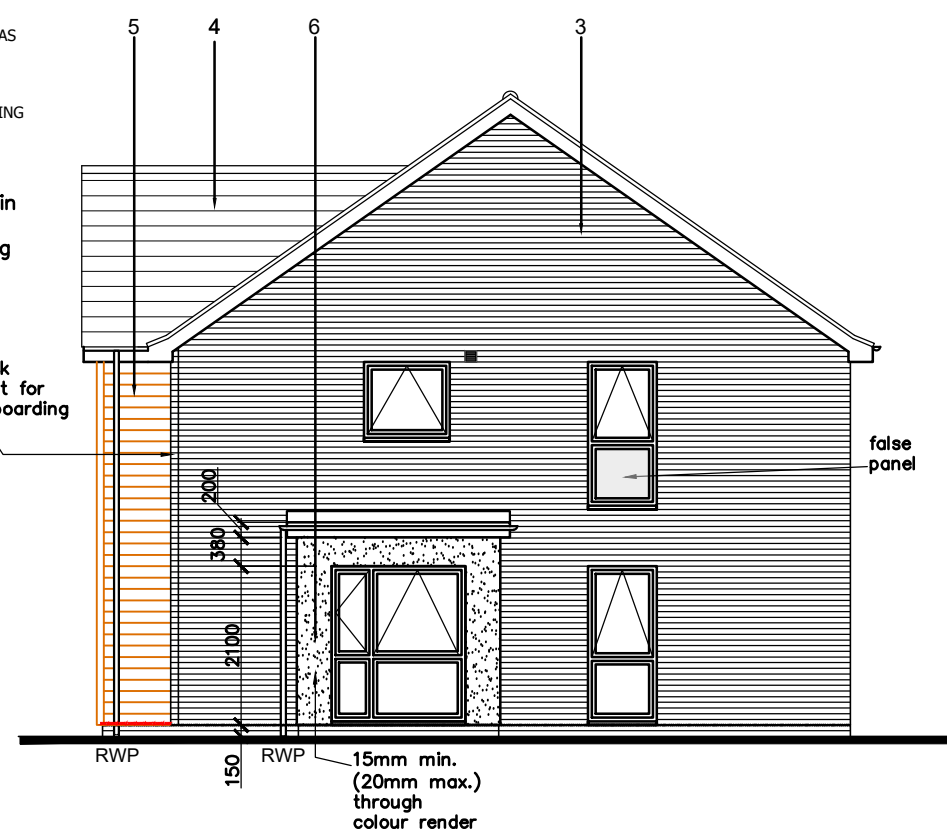
SIDE ELEVATION
