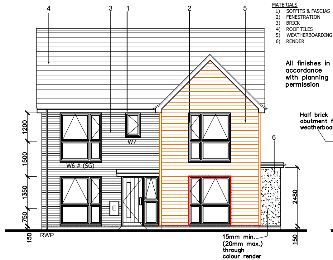
FRONT ELEVATION
