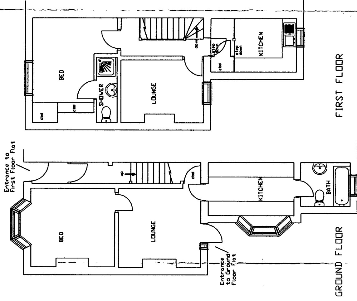
PROPOSED FLOORPLANS 1:100
