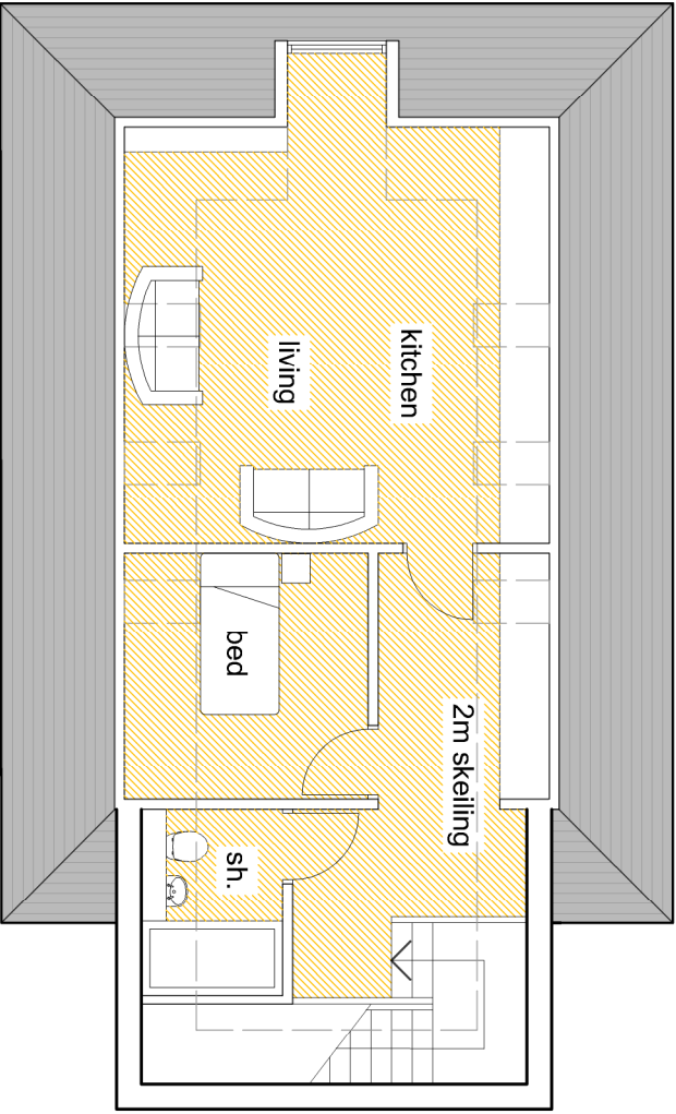
Proposed second floor plan Scale 1:100 @A3
