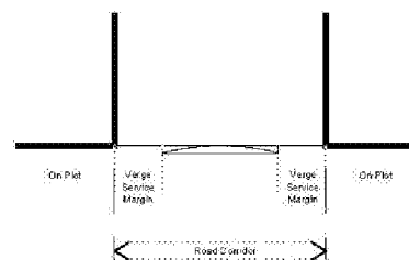
Shared Surface - Typical Section
