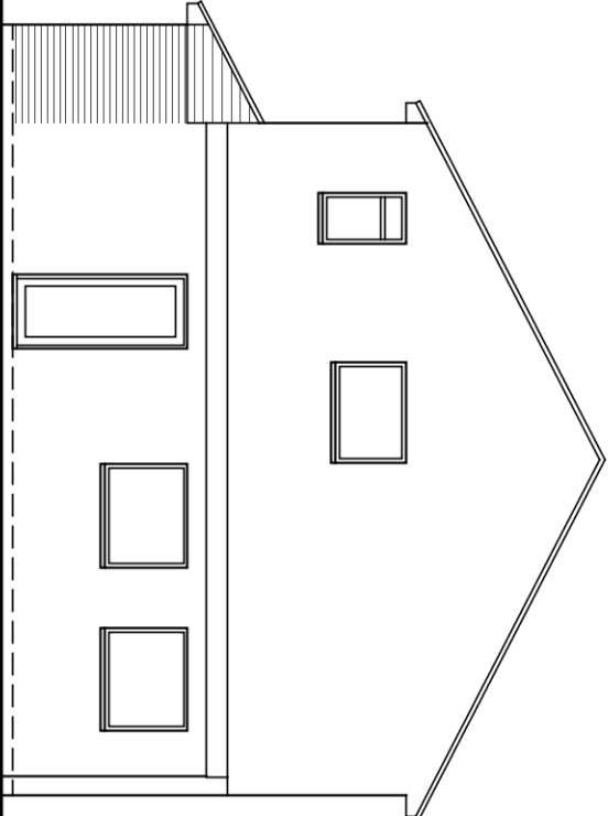
Side - West
