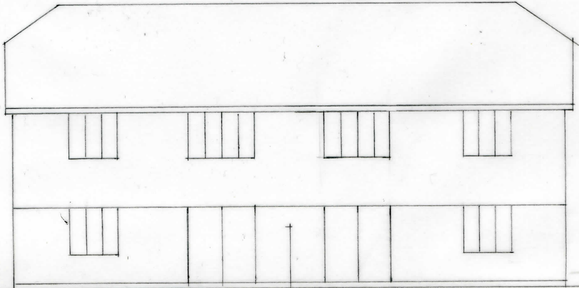
rear elevation
