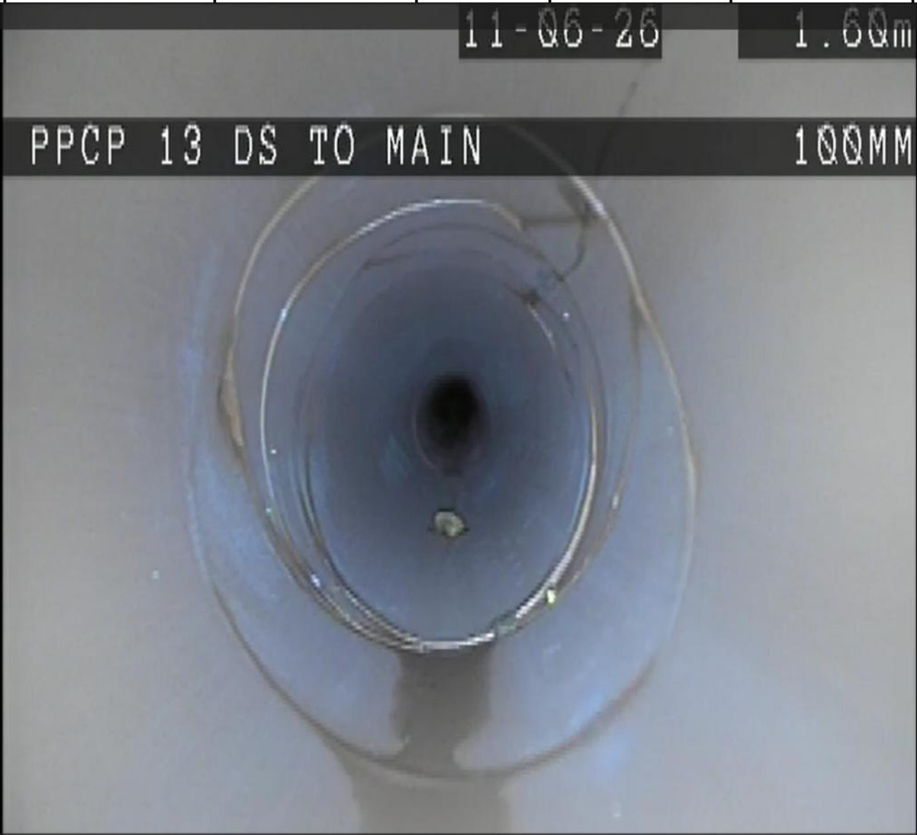
MULTIPLE CRACKS IN PIPE
