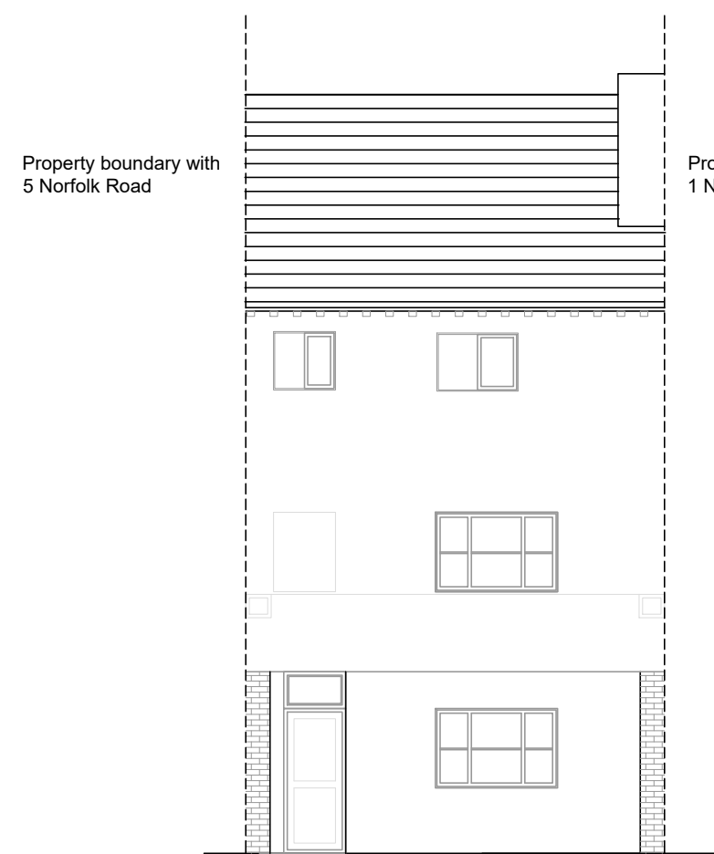
FRONT ELEVATION East
