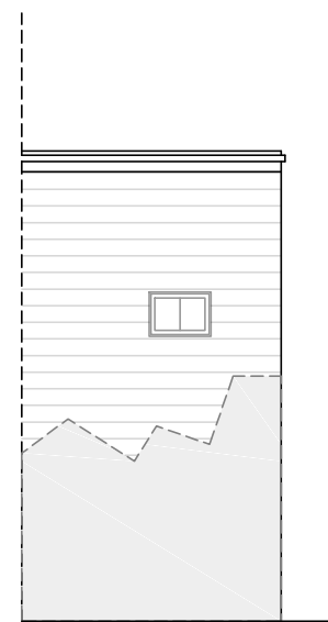
SIDE ELEVATION West
