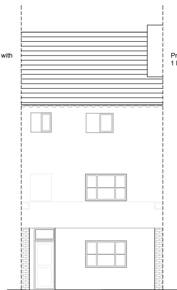
FRONT ELEVATION East
