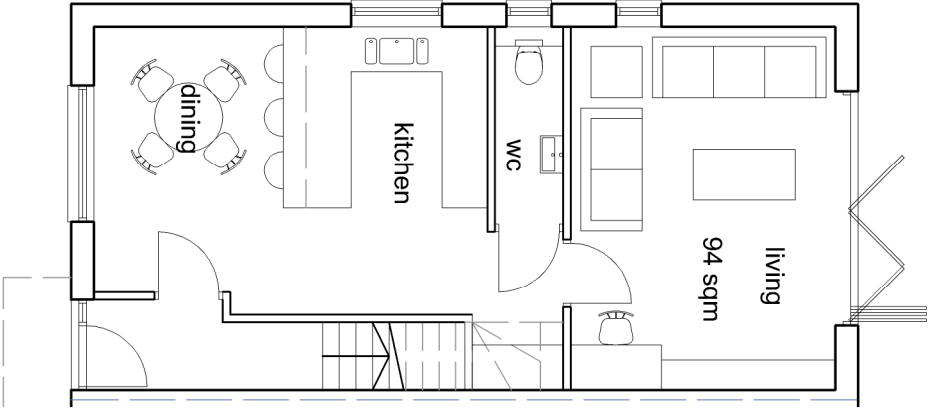
Proposed ground floor plan - 3 bed - units 15-20
