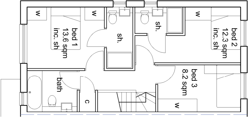
Proposed first floor plan - 3 bed - units 15-20
