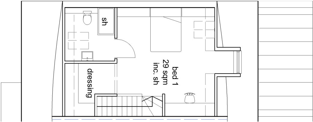
Proposed roof plan - 4 bed - units 11-14
