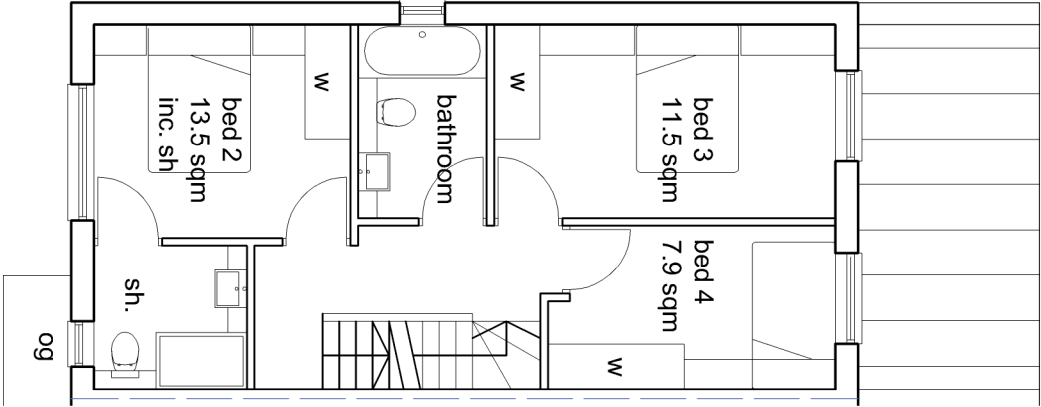
Proposed first floor plan - 4 bed - units 11-14
