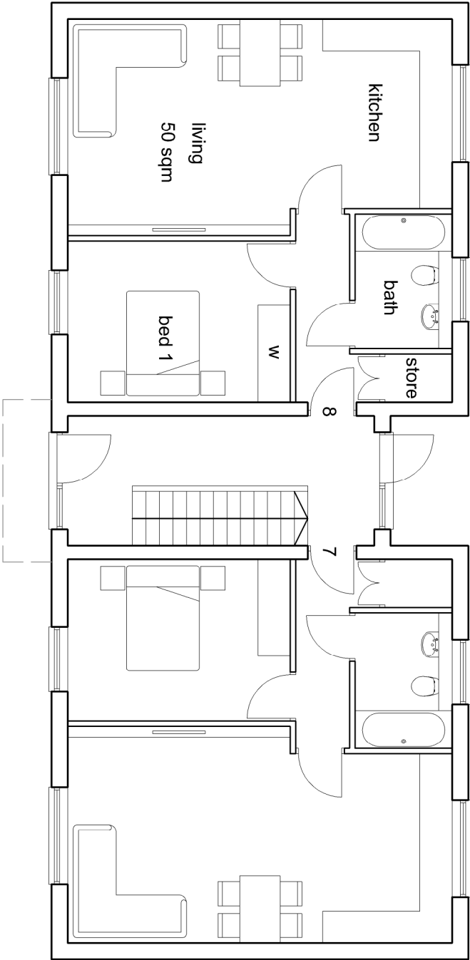
Proposed ground floor plan - 1 beds - units 7-10
