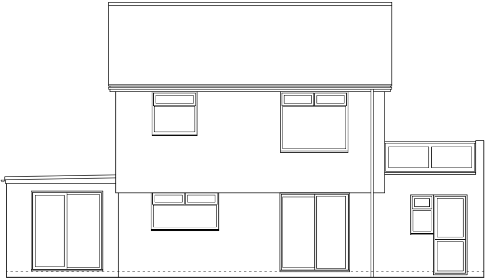
South Elevation
