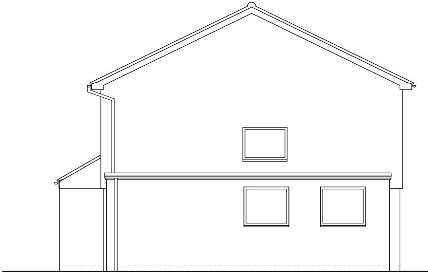
West Elevation
