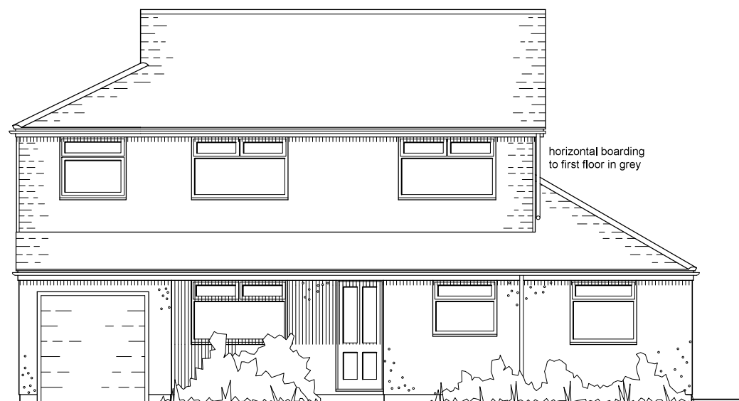
North Elevation
