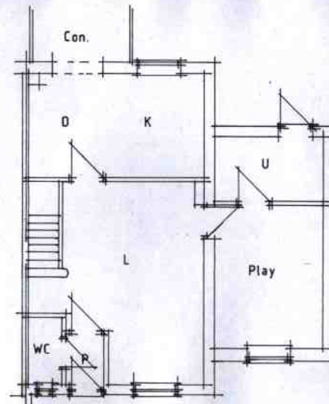
Extg ground floor 1:100
