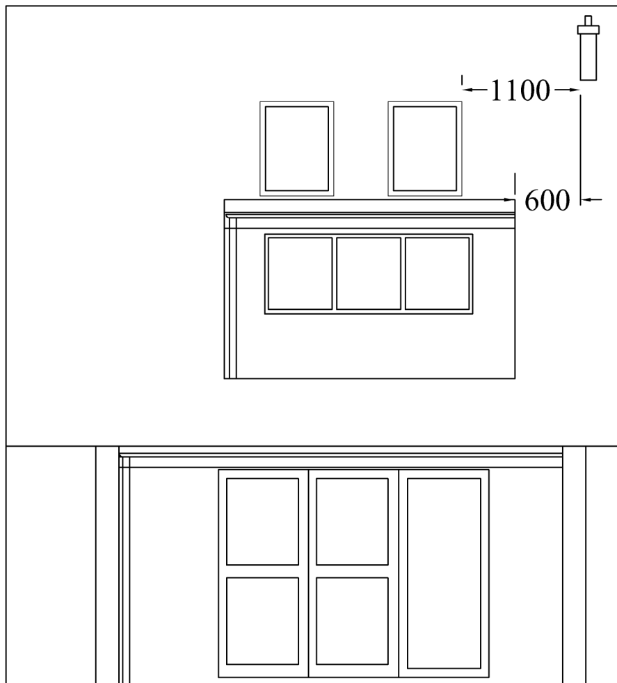
Rear Elevation
