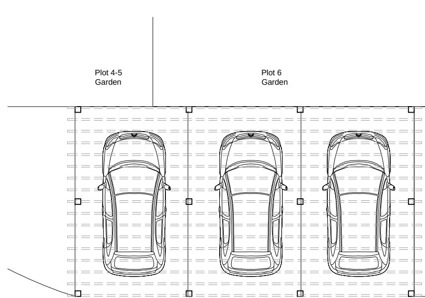
Plan Pergola
