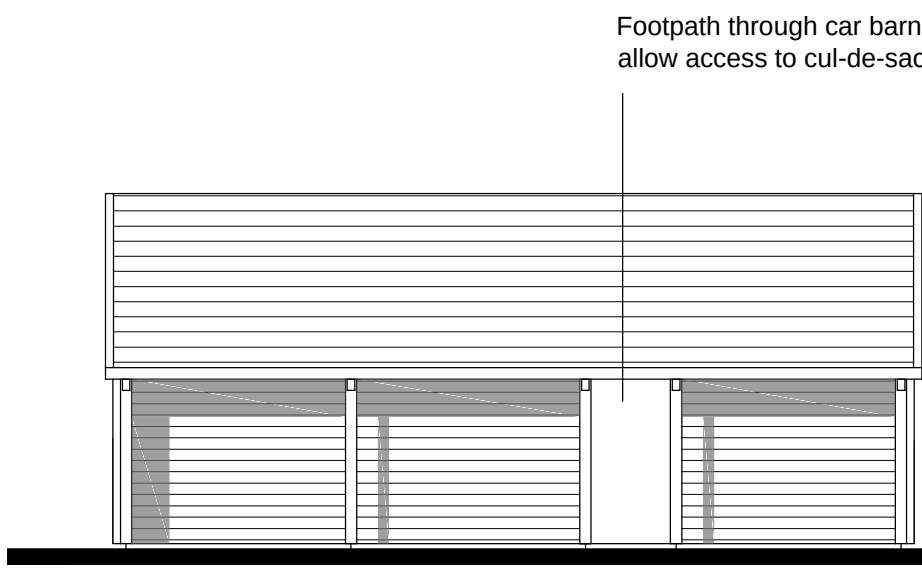
Front Elevation Triple Car Barn Plots: 1, 2 & 10
