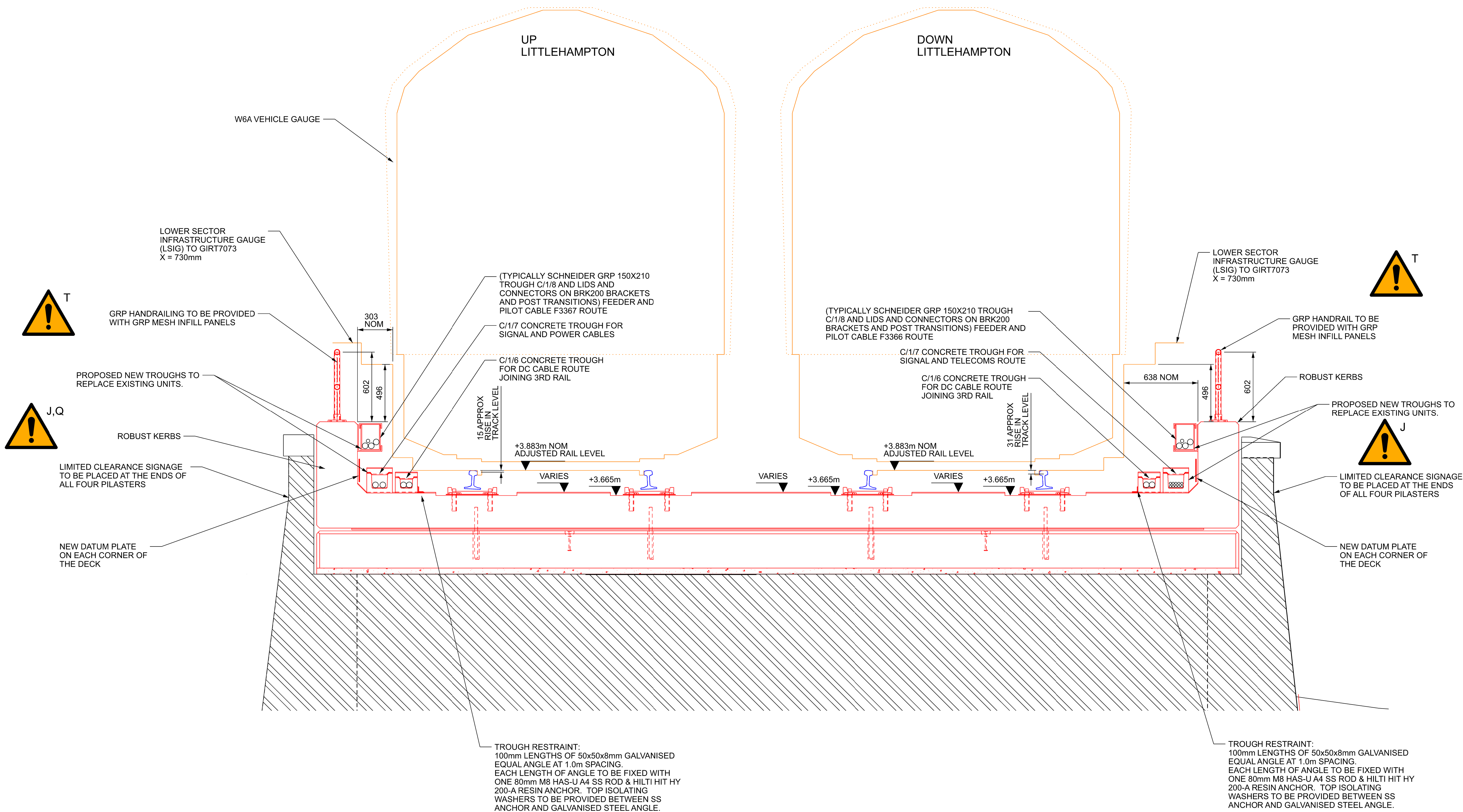
SECTION F-F STRUCTURAL CLEARANCE 1:20
