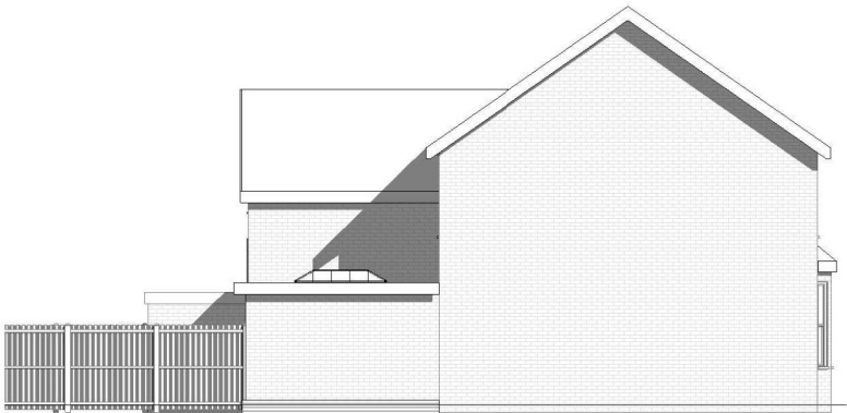
Proposed Elevation-Left side
