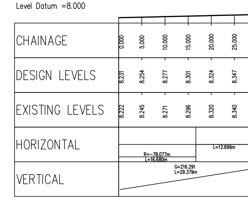
Proposed Longitudinal Section along MCL1 Scale H=1:500; V=1:100
