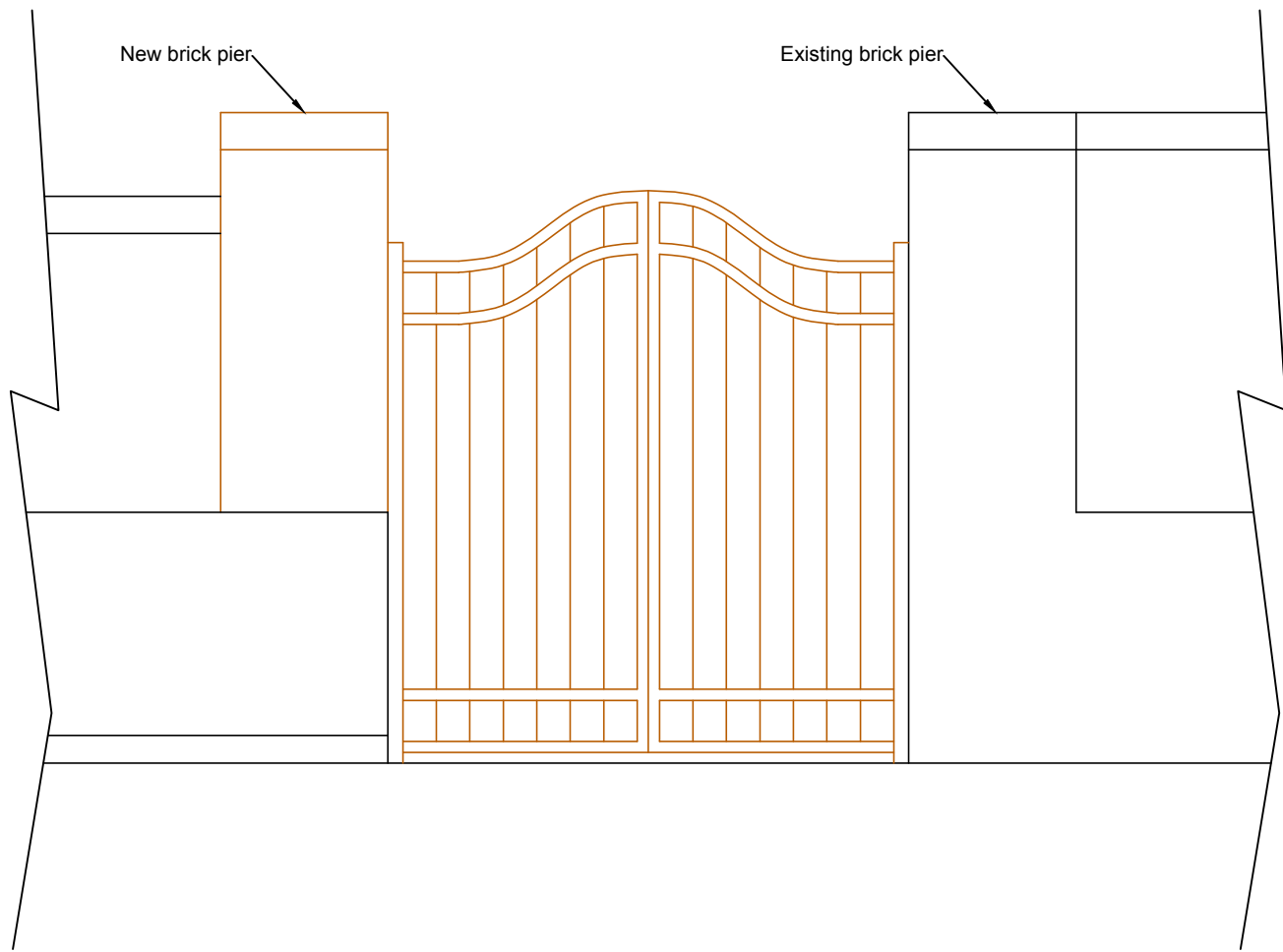
PROPOSED FRONT BOUNDARY WALL ELEVATION 1:20
