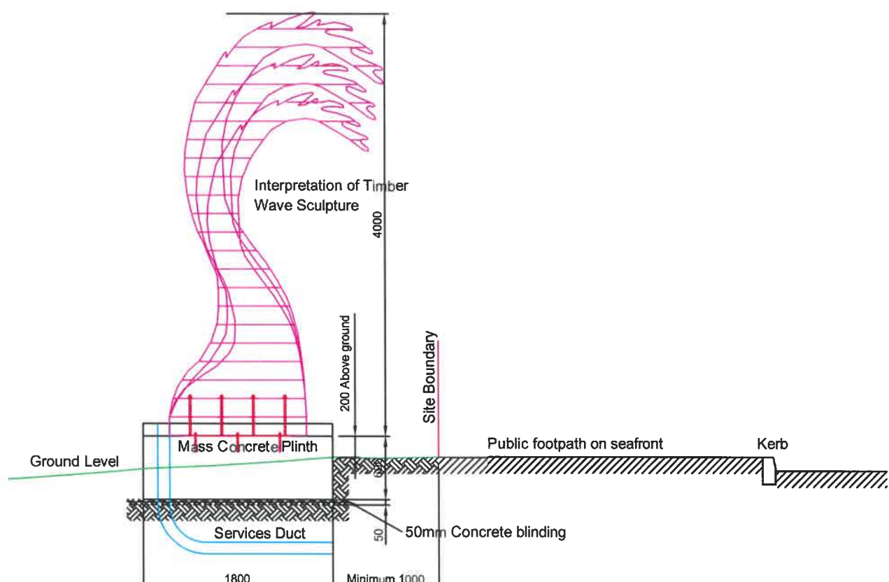
Section of Wave Sculpture
