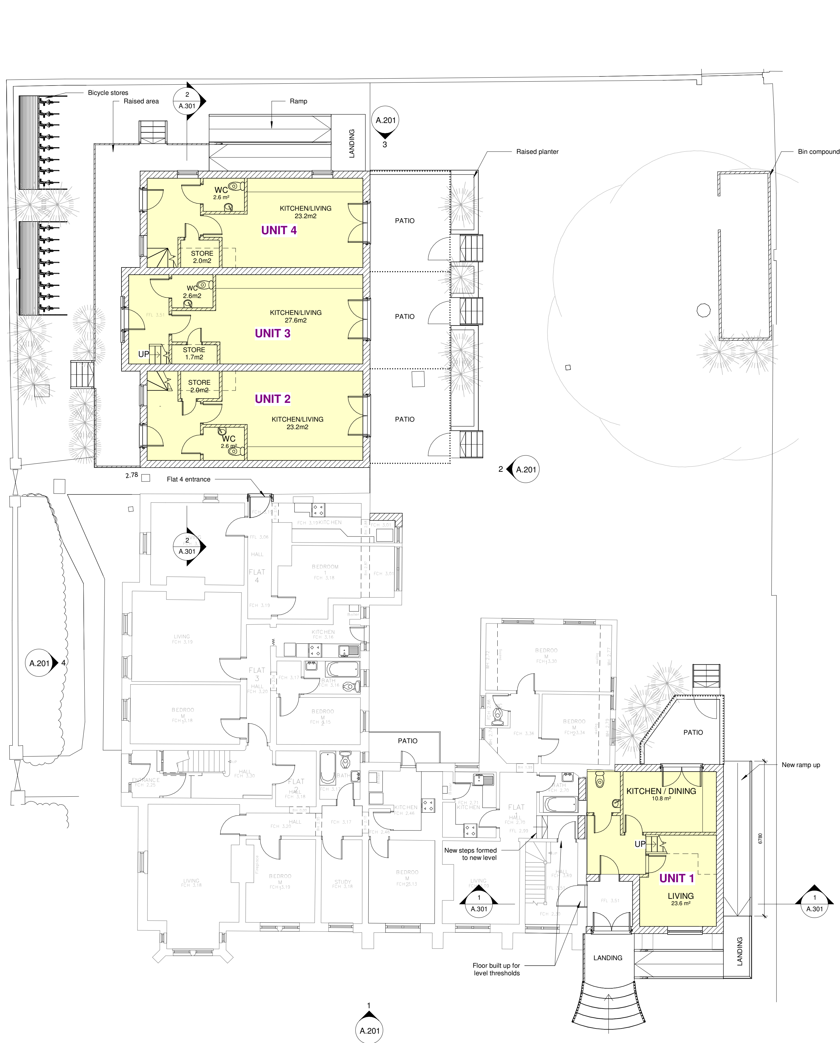
1 GROUND FLOOR 1 : 100
