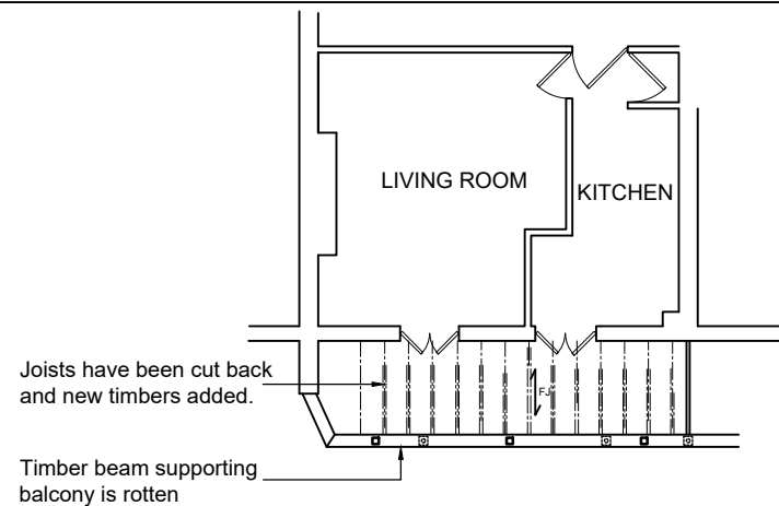
Existing First Floor Showing Balcony (1:100)
