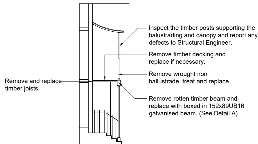
Proposed Section A-A (1:100)
