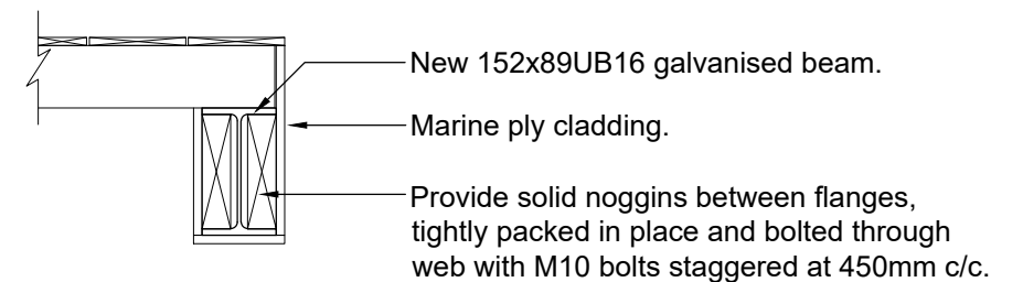
Detail A - Floor Joist to Beam Connection Detail (1:10)
