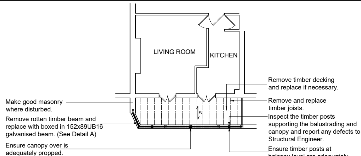
Proposed First Floor Showing Balcony (1:100)
