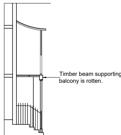
Existing Section A-A (1:100)
