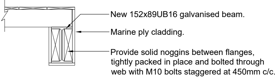
Detail A - Floor Joist to Beam Connection Detail (1:10)
