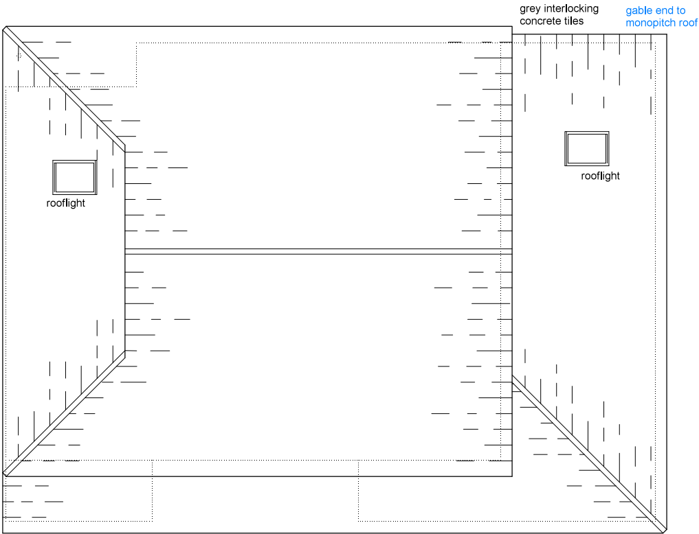
Roof Plan
