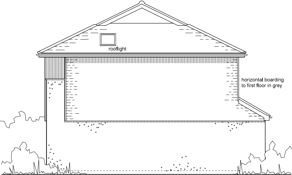
East Elevation
