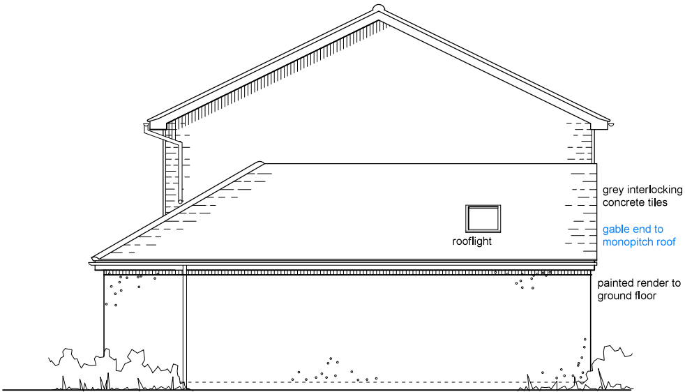
West Elevation
