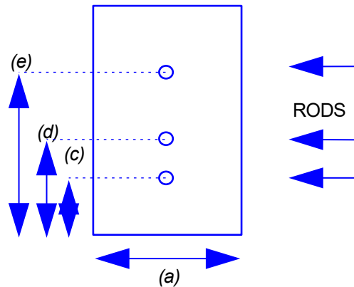
EXISTING TIMBER TO BE DRILLED IN SITU
