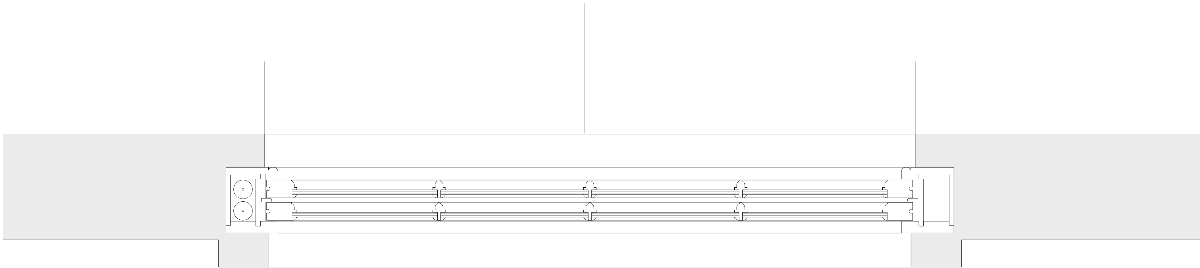
WT17 SASH REPLACEMENT SASH WINDOW ELEVATION - 1:5@A0
