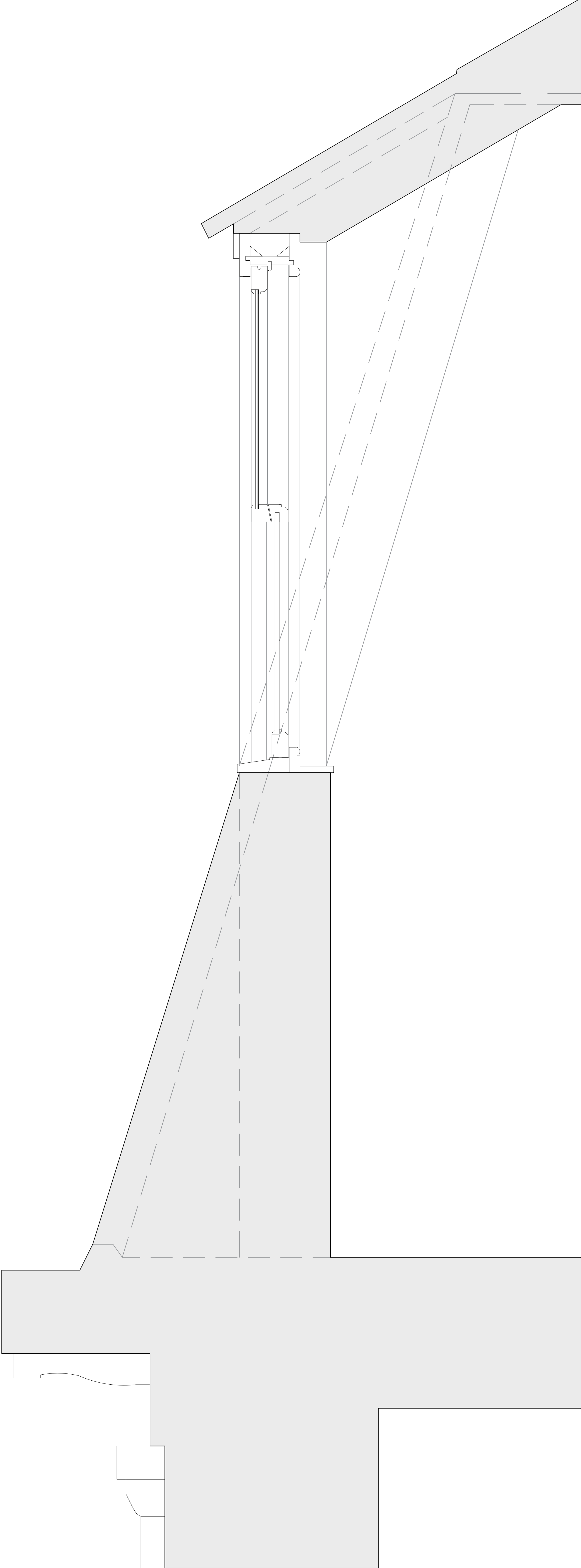
WT17 SASH REPLACEMENT SASH WINDOW SECTION - 1:5@A0
