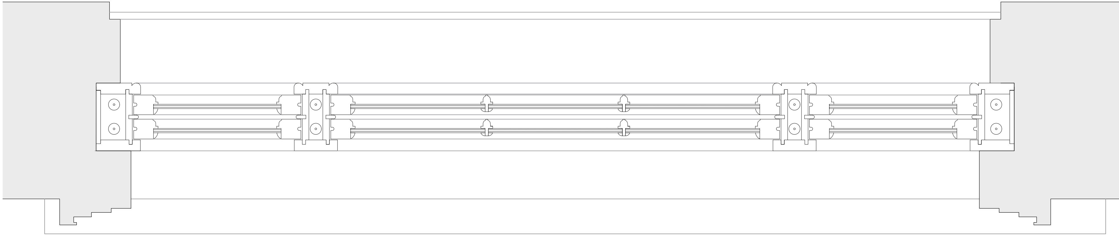
WT16 SASH REPLACEMENT SASH WINDOW PLAN - 1:5@A0
