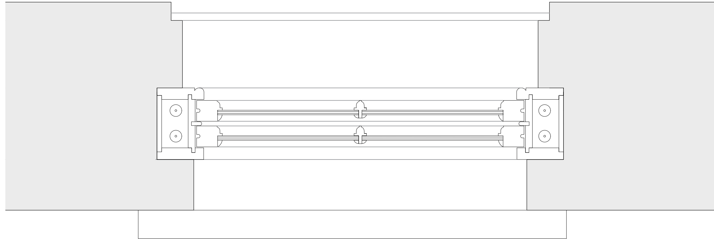
WT10 SASH REPLACEMENT SASH WINDOW PLAN - 1:5@A0
