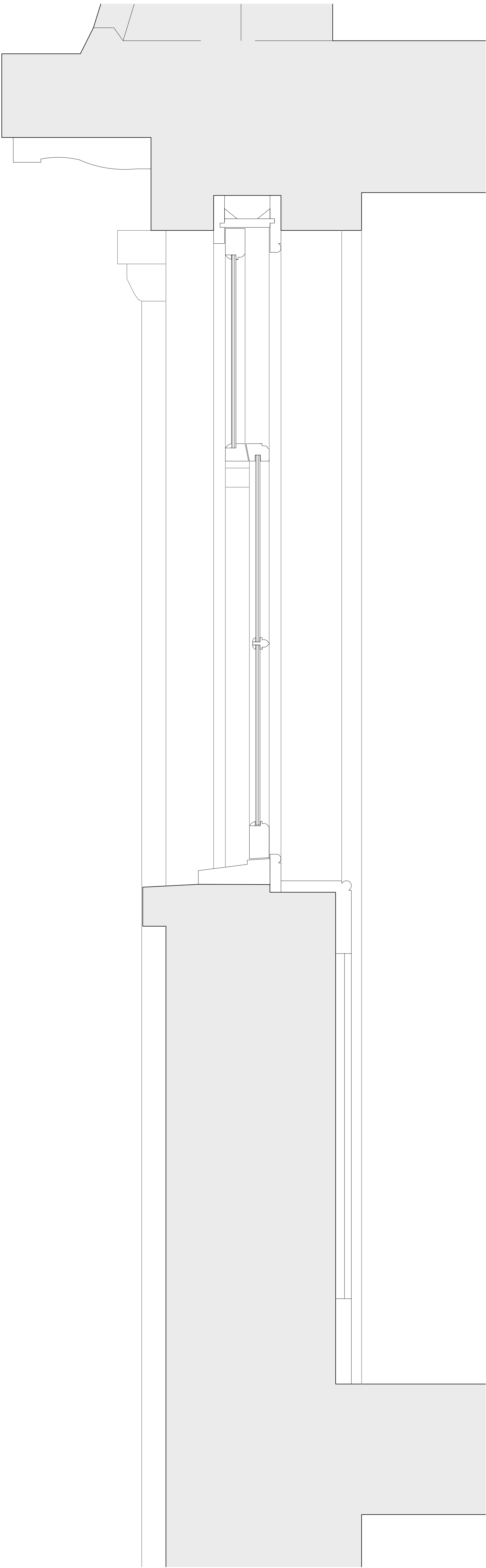
WT10 SASH REPLACEMENT SASH WINDOW SECTION - 1:5@A0
