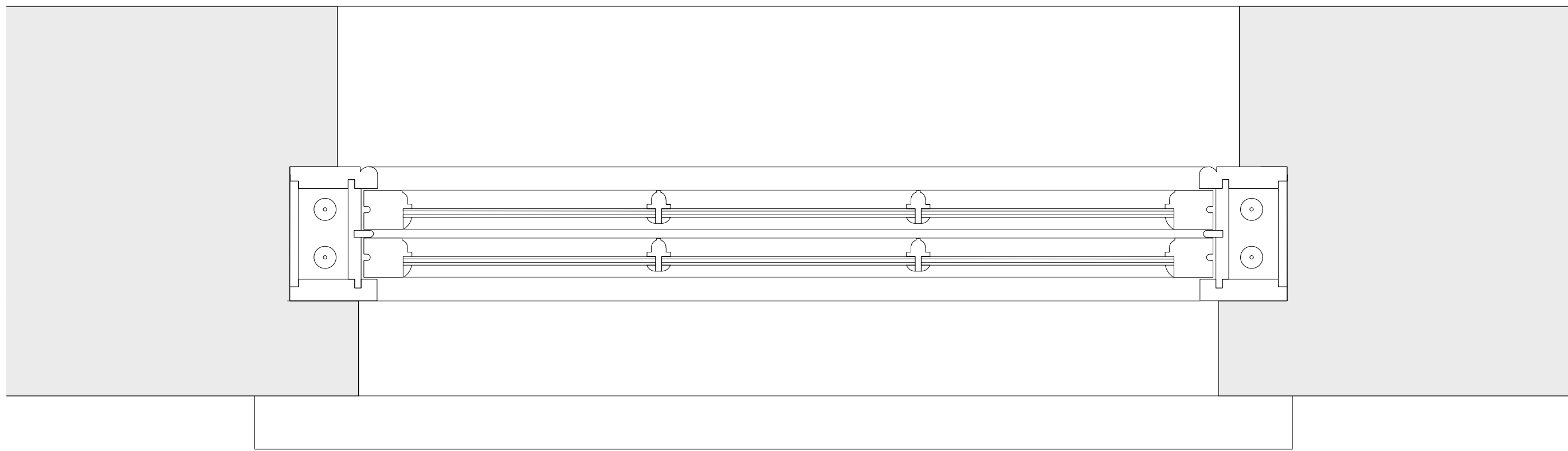
WT04 SASH REPLACEMENT SASH WINDOW PLAN - 1:5@A0
