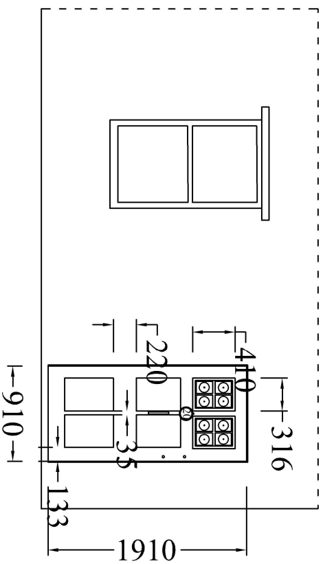
Front Elevation
