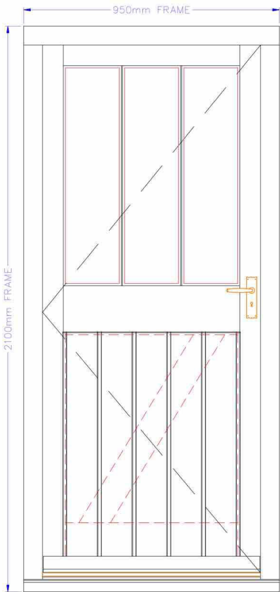
FRONT ELEVATION
