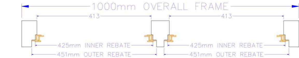
PLAN
