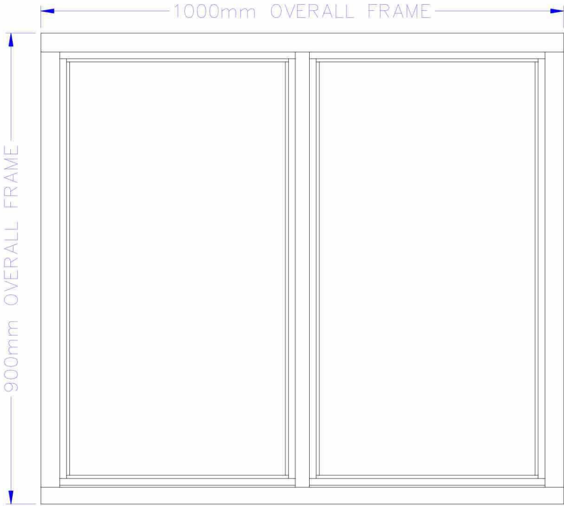
FRONT ELEVATION
