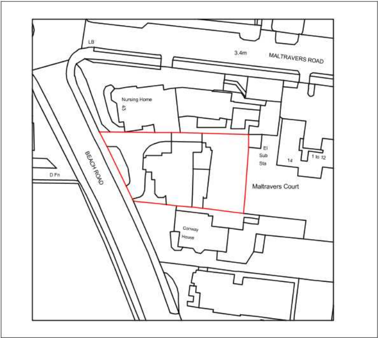
LOCATION PLAN 1:1250
