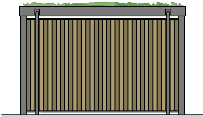
Left / Right Elevation
