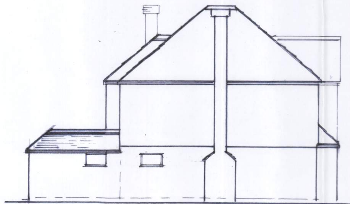
PROP. EAST ELEVATION 1:100
