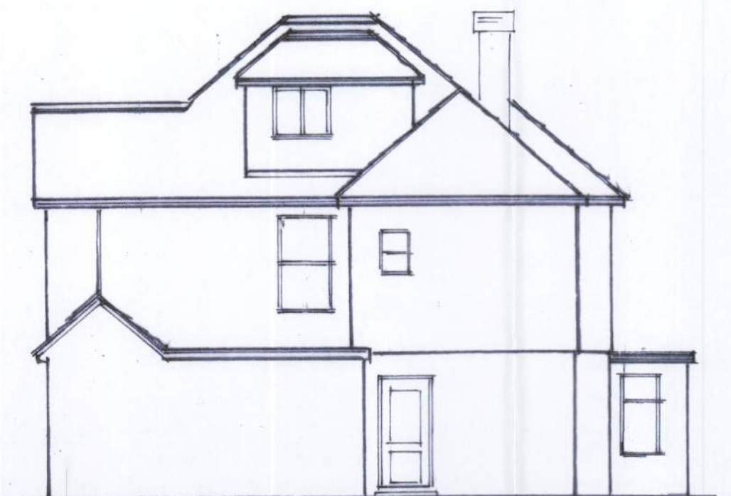
EXTG. WEST ELEVATION 1:100
