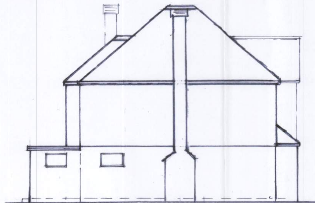
EXTG. EAST ELEVATION 1:100
