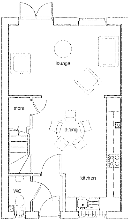
Plot 60 3 - Bedroom House Ground Floor Plans
