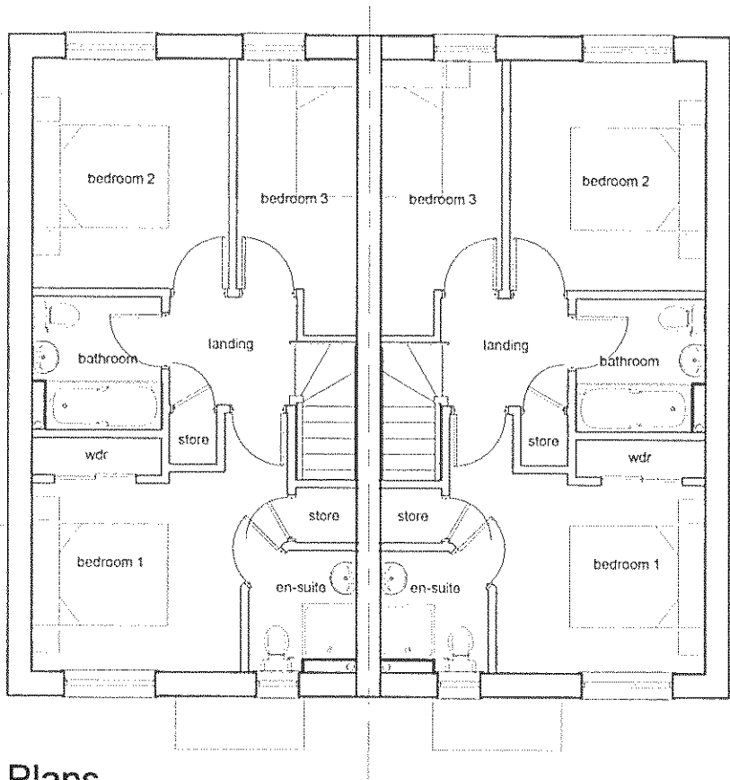
First Floor Plans
