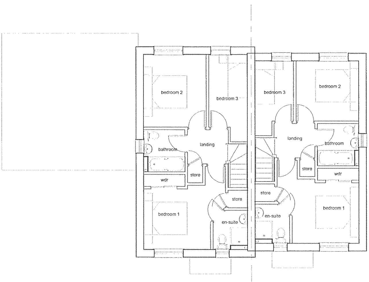
First Floor Plans
