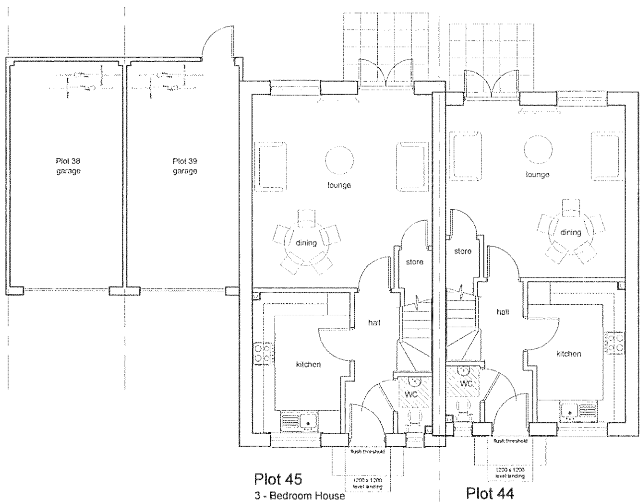
Ground Floor Plans
